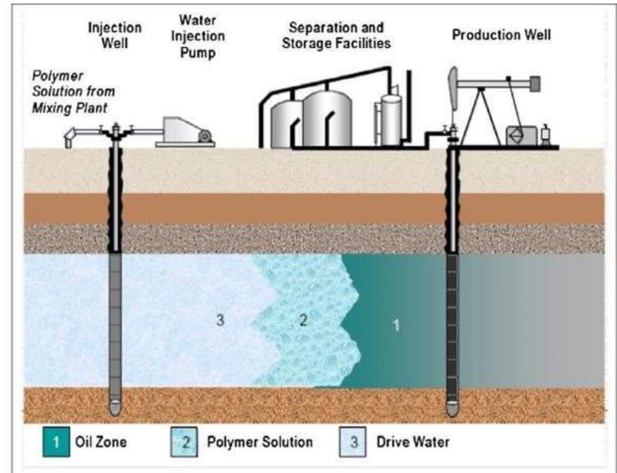
EOR - Water & Polymer Flooding
